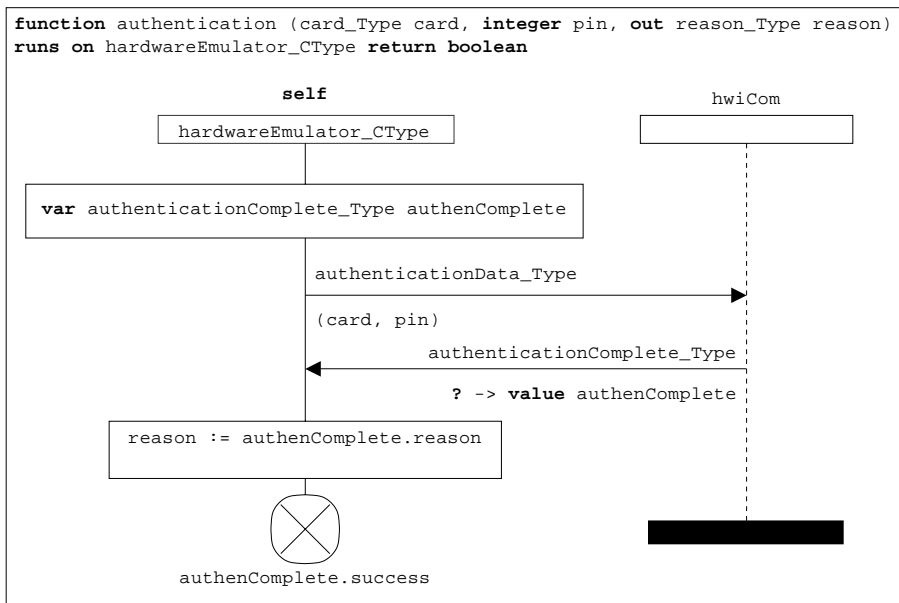
Figure 18. GFT representation of function authentication
