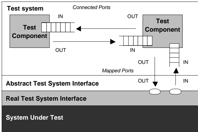
Figure 3. Conceptual view of a TTCN-3 test system
