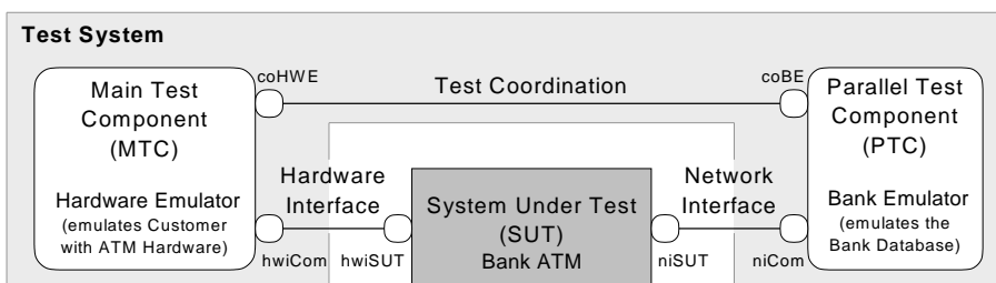
Figure 7. Test system for the ATM example
