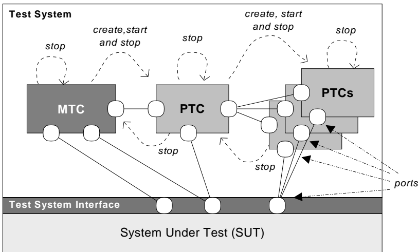
Figure 2. Dynamic and concurrent test system
