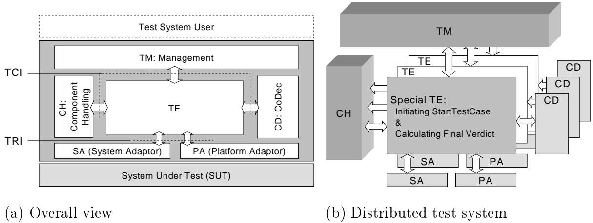
Figure 21. General structure of TTCN-3 test systems
